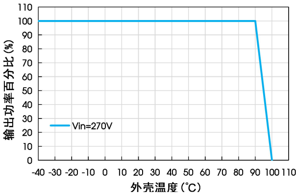
VRF3D24/28QB-100WR3-N温度降额曲线
