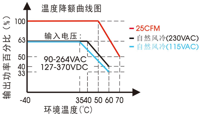
LOF450-20B12/15/18/19-CF (满载 400W 带 25CFM 风扇)
