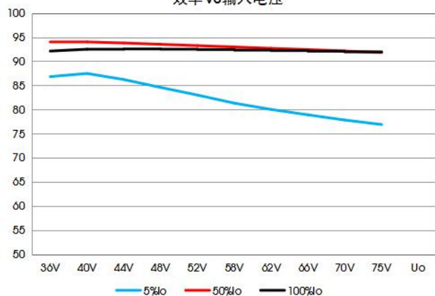
VCF4805EBO-150W(F)R3-N 效率VS输入电压
