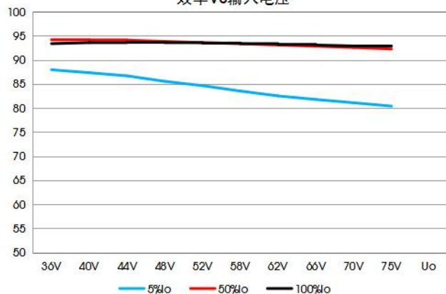
VCF4812EBO-150W(F)R3-N 效率VS输入电压
