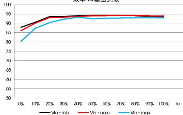
VCF4812EBO-150W(F)R3-N 效率VS输出负载
