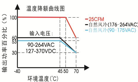
LOF750-20B24/27/36/48/54 (满载 750W 带 25CFM 风扇)
