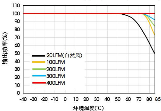
URF4824QB-100WFR3 温度降额曲线 (Vin=24V)
