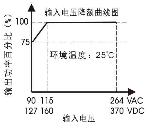
LOF550-20Bxx-C(-CF)输入电压降额
